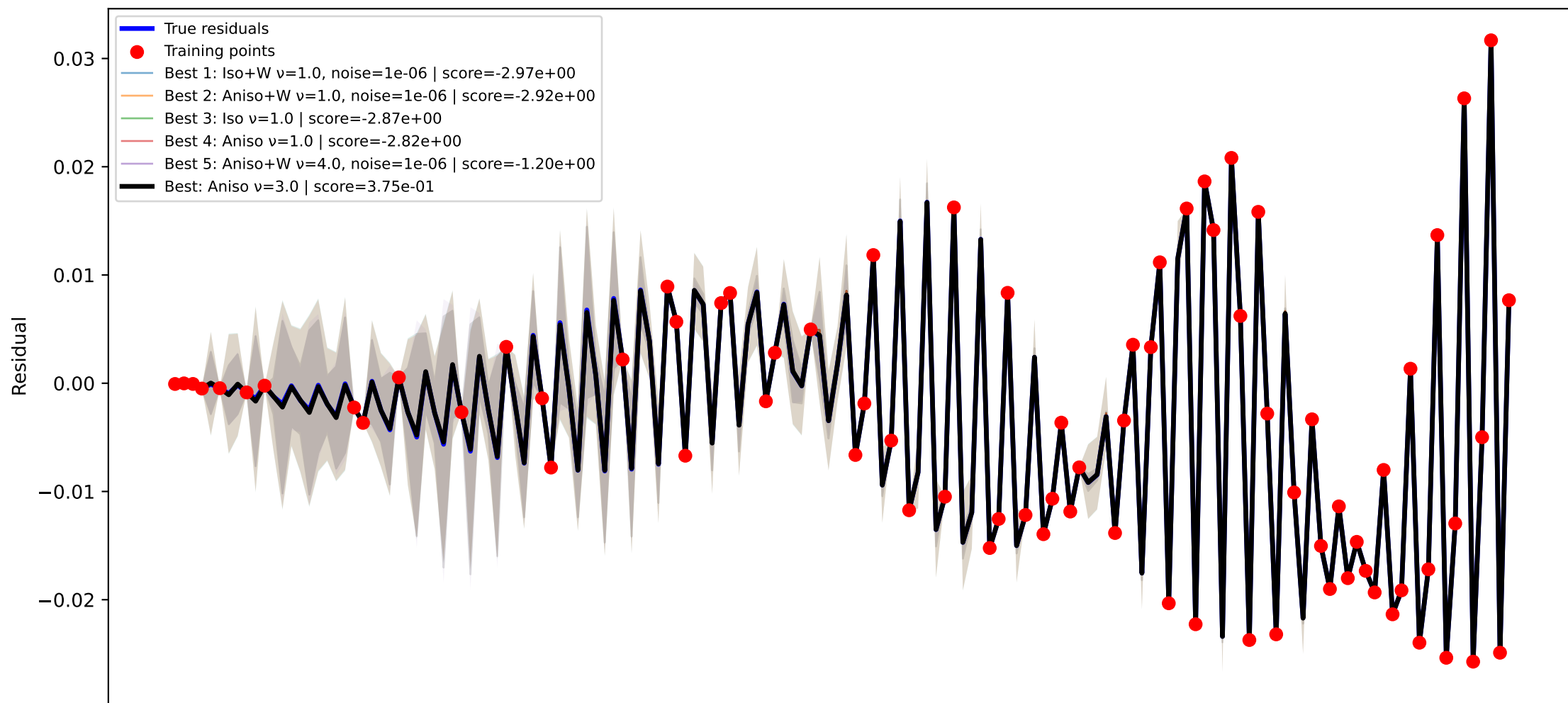
GPR kernel comparison node=49 RMSE=6.589e-05, train RMSE=2.699e-11
